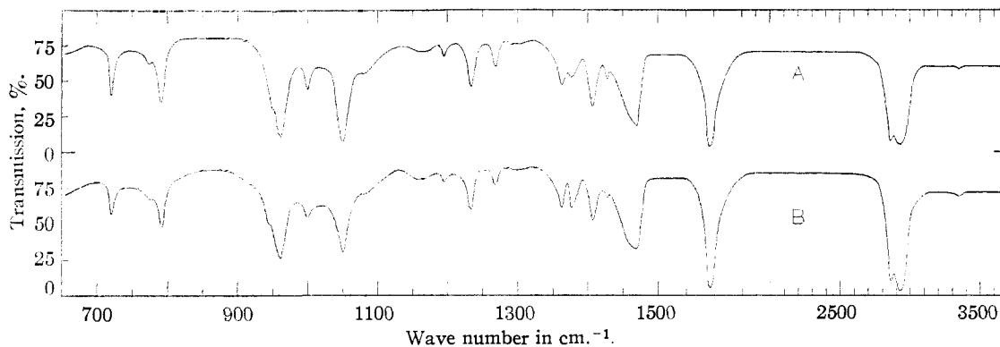
Fig. 1.—A, Polymer from adipyl chloride and hexamethylenedithiol; B, polymer from biallyl and dithioladipic acid.
